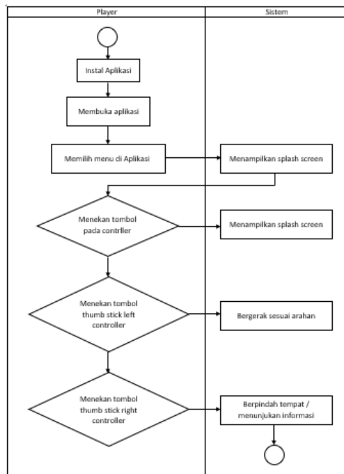
Gambar 2. Flowchart VR
